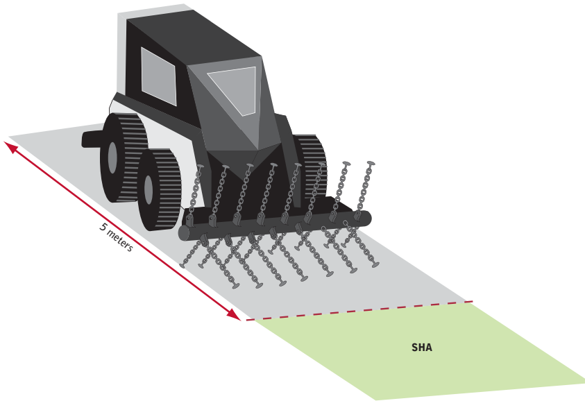
Figure 10 | On-site testing
